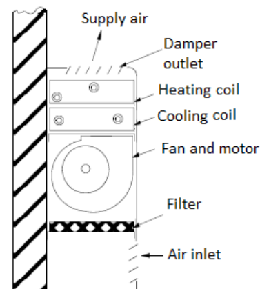
Vertical Fan Coil Unit
